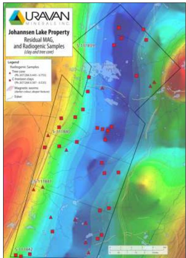
Figure 4—JL project map showing positive tree-core, clay and vegetation anomalies
